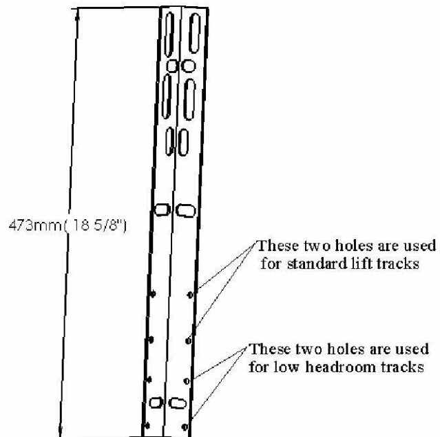
Figure 5.B: Angle for track 1 3/4" (44.5 mm)
