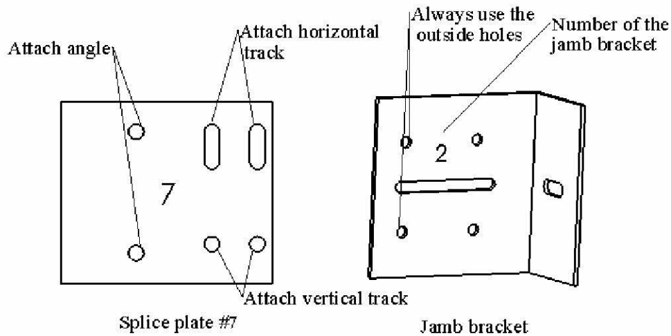
Figure 5.A: Splice plate and jamb bracket
